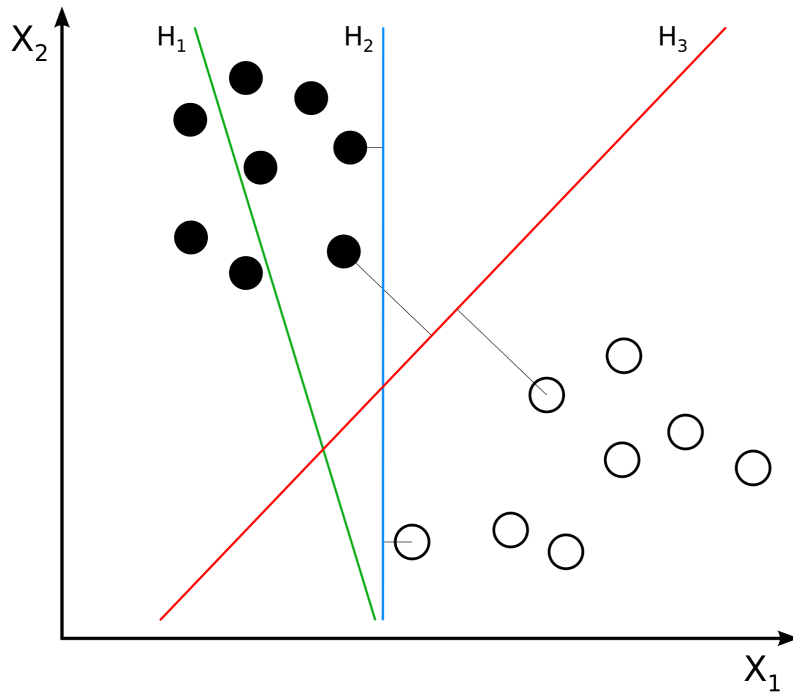
Figure 1: Three different examples ( H_1, H_2, H_3 ) of how a support vector machine could separate the data into two regions (5)
