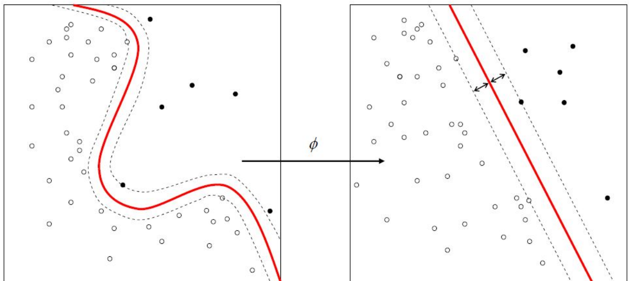
Figure 2: A kernel is used to transform a nonlinear function into a linearly separable function (5)
